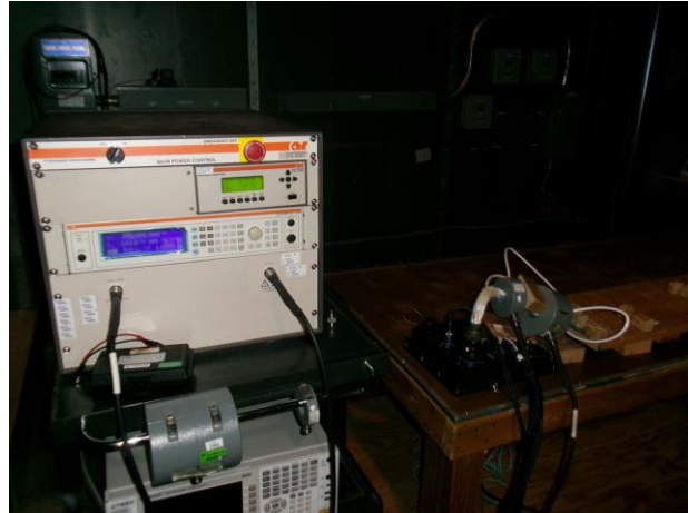
08 - CS114 Test, Ethernet
