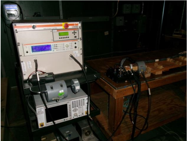
07 - CS114 Test, Hot Lead Only
