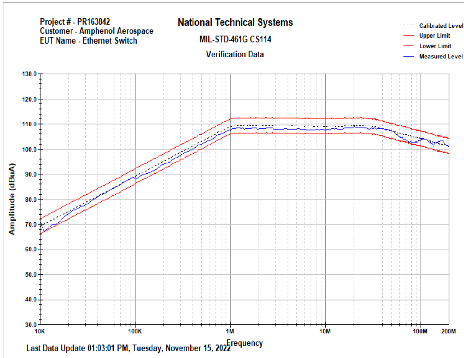
03 - Verification Data
