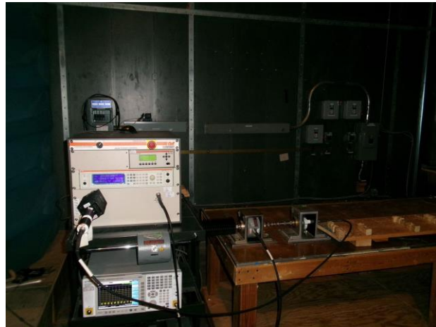
04 - CS114 Calibration
