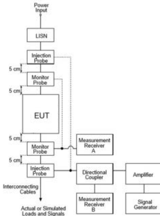
Figure 5.3-5: CS114 Bulk Cable Injection Evaluation
