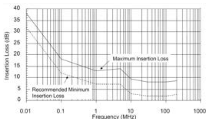
Figure 5.3-2: CS114 Maximum Insertion Loss for Injection Probes
