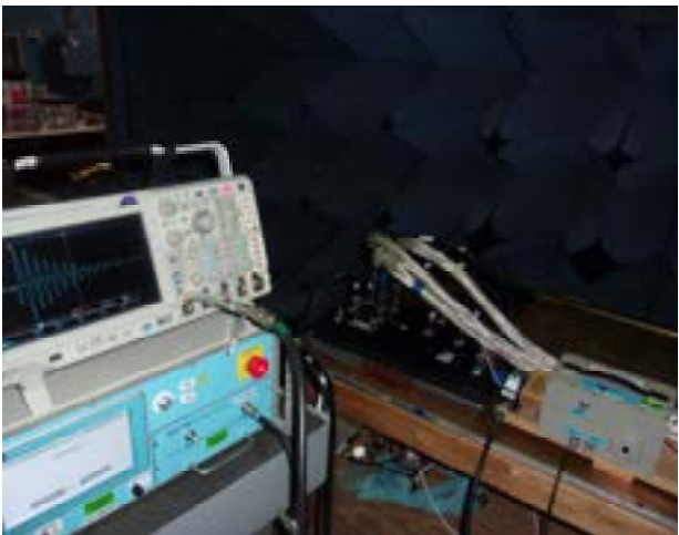
CS116 Power Bundle
