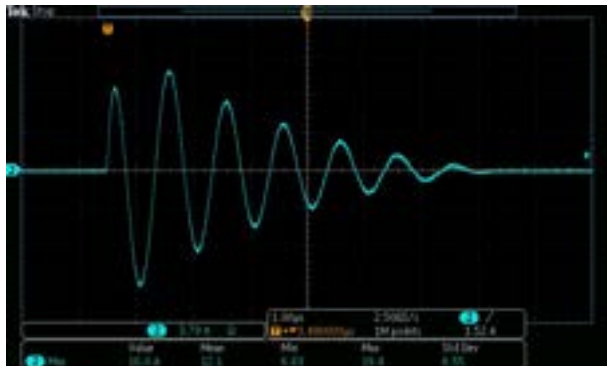
CS116 Test: 1MHz
