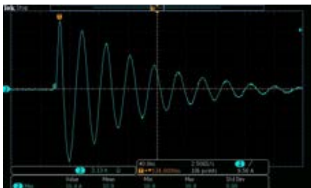
CS116 Monitor Probe Calibration: 30MHz
