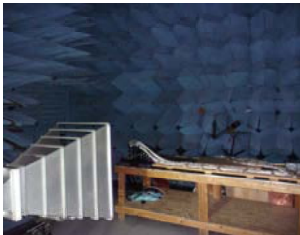
RE102, 200MHz-1GHz Horizontal Position 1
