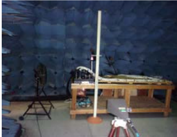
RS103, 8-18GHz, Vertical Position 2
