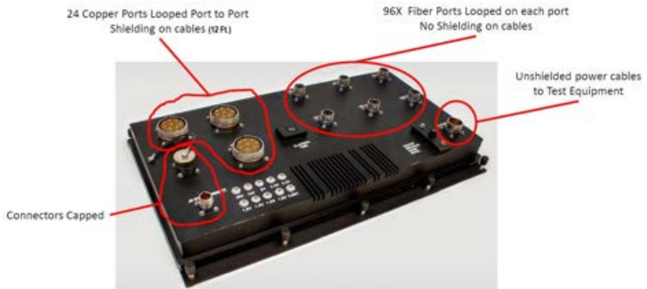
Figure 3.2-1: EUT Setup Overview
