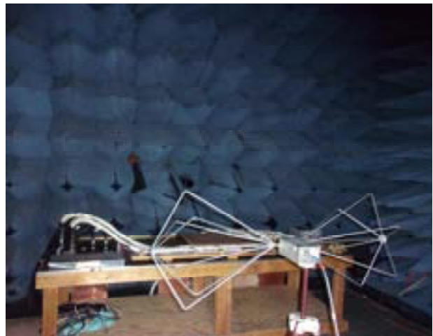
RE102, 30-200MHz Horizontal
