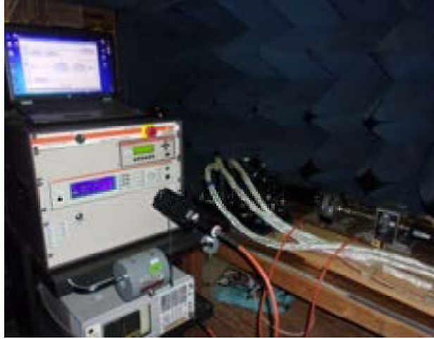
CS114 Verification
