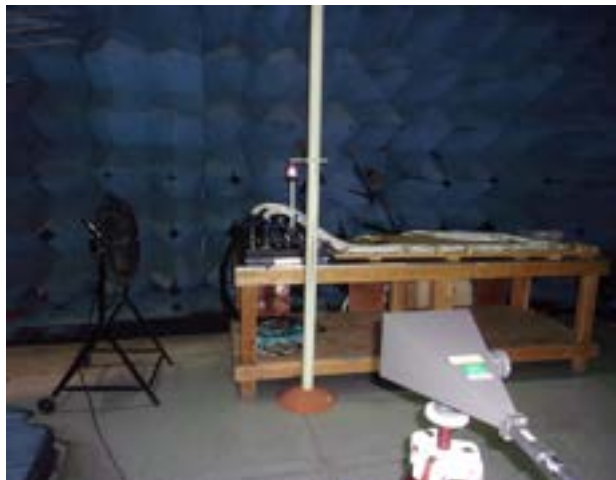
RS103, 6-8GHz Vertical
