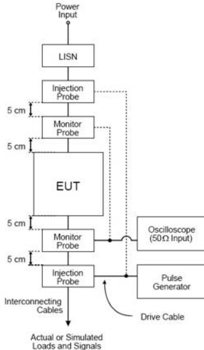
Figure 5.4-3: CS115 Bulk Cable Injection
