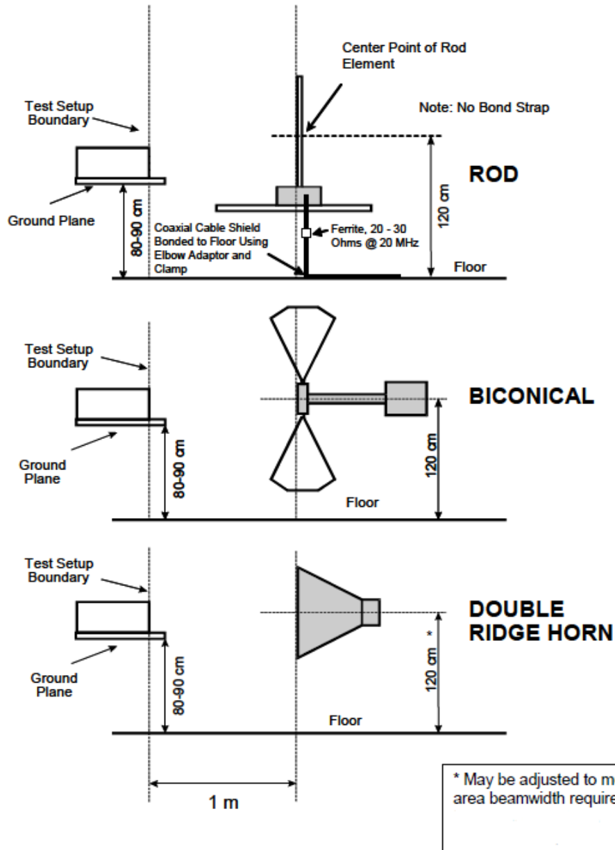
Figure 5.2-3: Antenna Positioning
