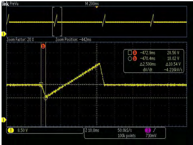
Repetitive Normal Transient - V1, T1, V2
